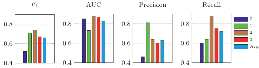
Fig. 5. Per-class MDS-UPDRS gait score estimation performance of our method.
